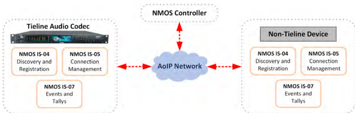
Overview of Tieline NMOS codec integration
